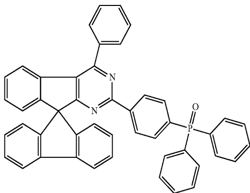
Chemical Formula 1-51
