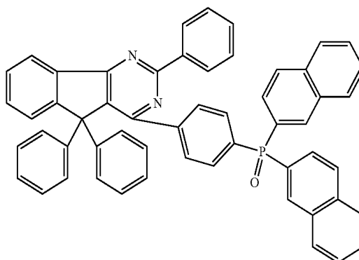
Chemical Formula 2-39
