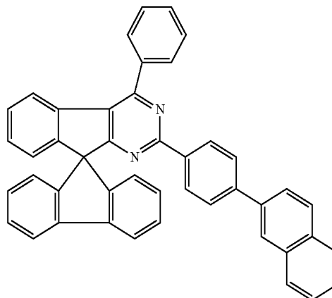
Chemical Formula 1-64
