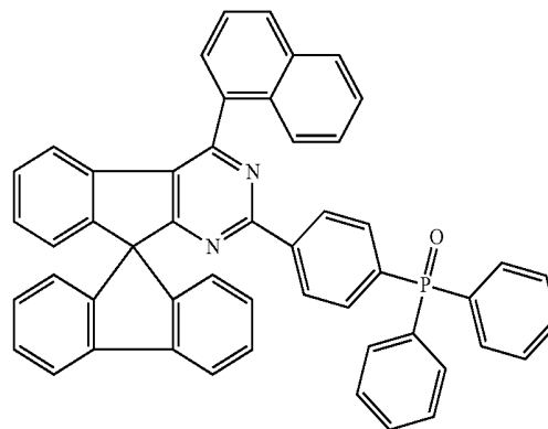
Chemical Formula 1-52
