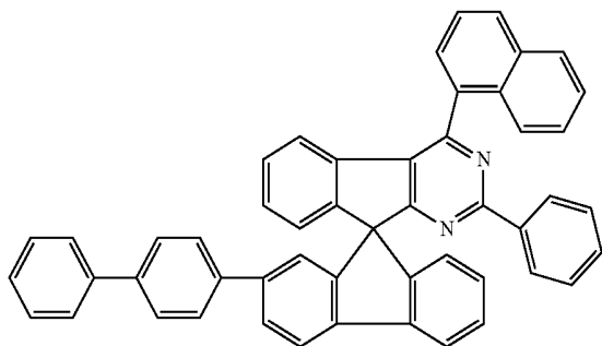
Chemical Formula 1-32
