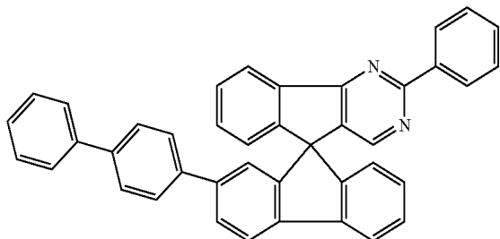
Chemical Formula 1-6
