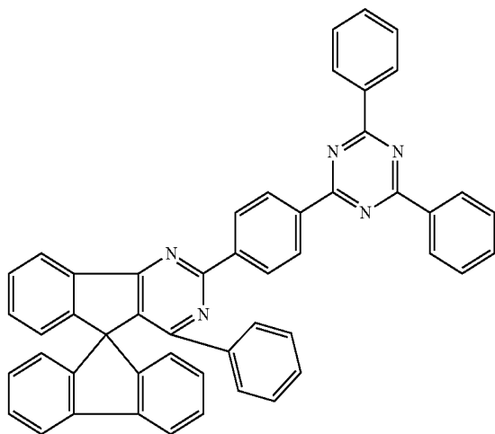
Chemical Formula 1-90
