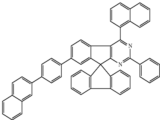
Chemical Formula 1-41
