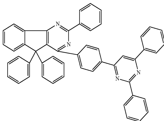
Chemical Formula 2-45
