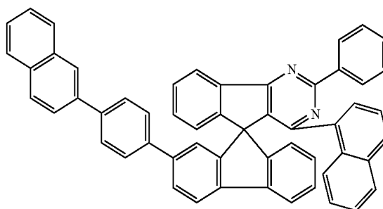
Chemical Formula 1-37
