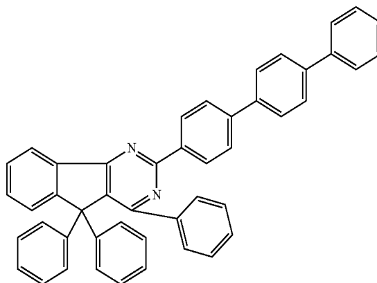
Chemical Formula 2-25
