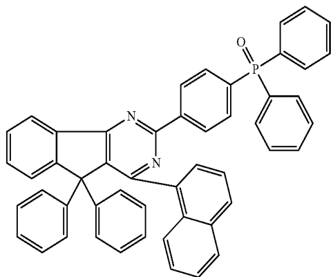
Chemical Formula 2-21
