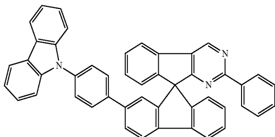
Chemical Formula 1-15
