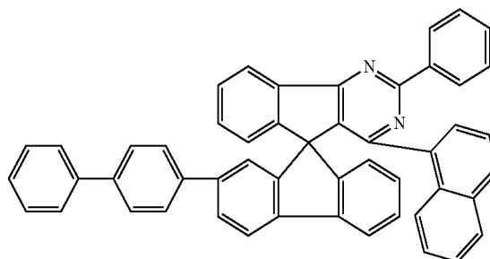
Chemical Formula 1-31
