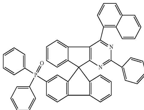
Chemical Formula 1-44
