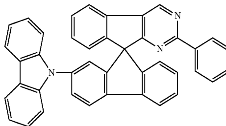
Chemical Formula 1-3
