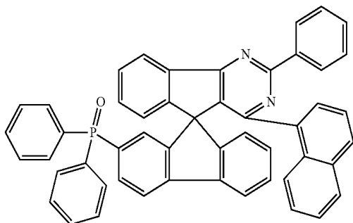
Chemical Formula 1-43
