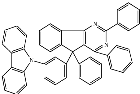
Chemical Formula 2-3
