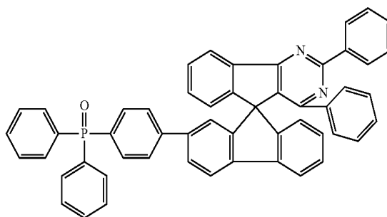
Chemical Formula 1-45
