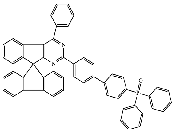
Chemical Formula 1-56
