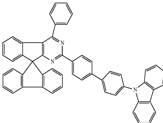
Chemical Formula 1-71
