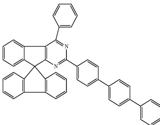
Chemical Formula 1-60
