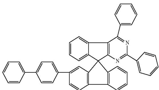
Chemical Formula 1-8
