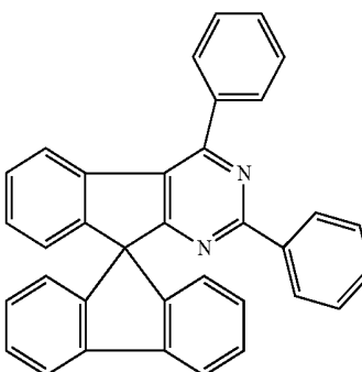
Chemical Formula 1-8
