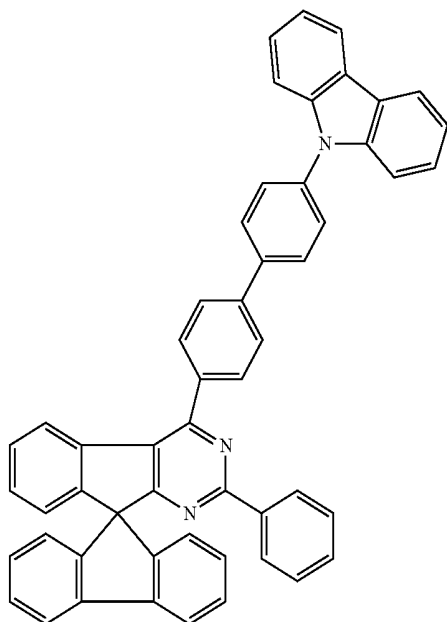
Chemical Formula 1-89
