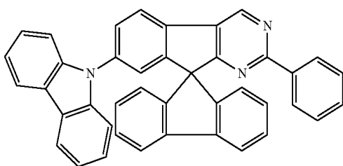
Chemical Formula 1-19
