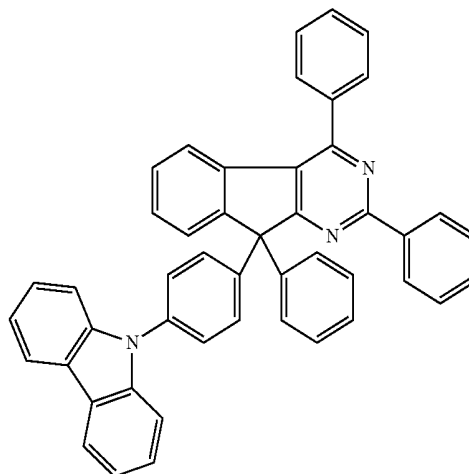
Chemical Formula 2-10
