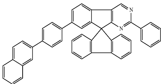
Chemical Formula 1-26
