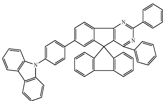
Chemical Formula 1-19
