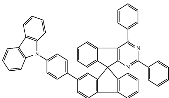
Chemical Formula 1-17
