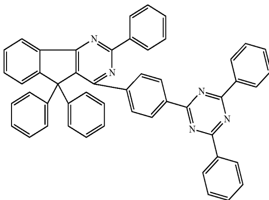
Chemical Formula 2-43
