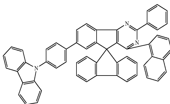
Chemical Formula 1-35
