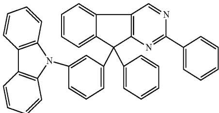
Chemical Formula 2-3
