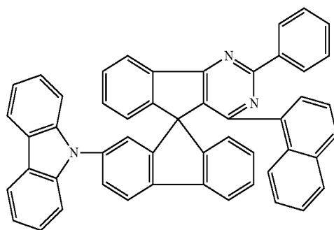
Chemical Formula 1-29
