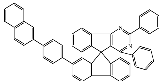
Chemical Formula 1-23
