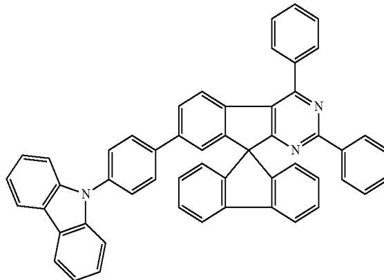
Chemical Formula 1-20
