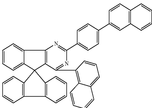
Chemical Formula 1-65
