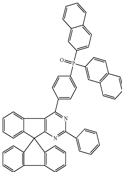
Chemical Formula 1-79
