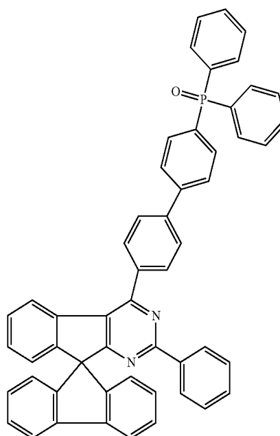
Chemical Formula 1-80
