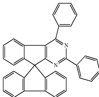
Chemical Formula 1-8
