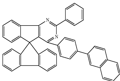
Chemical Formula 1-83
