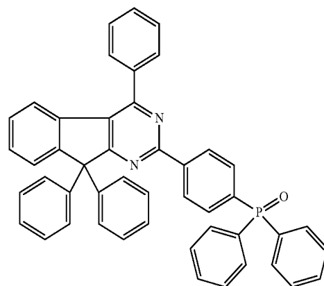
Chemical Formula 2-20
