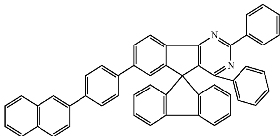
Chemical Formula 1-27
