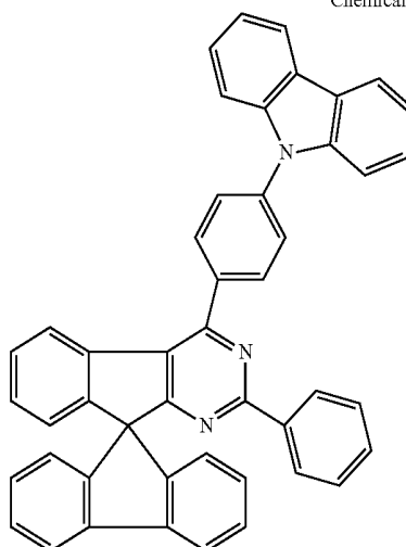
Chemical Formula 1-86
