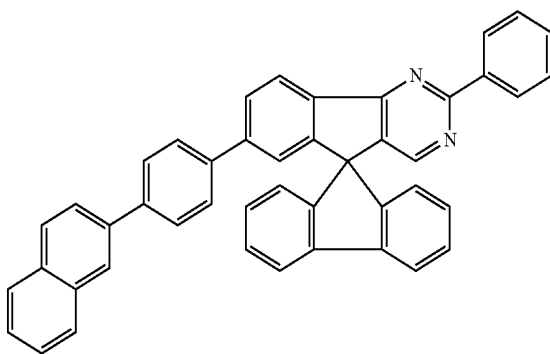
Chemical Formula 1-25
