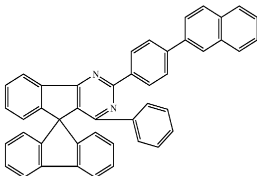
Chemical Formula 1-63
