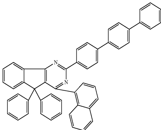
Chemical Formula 2-27
