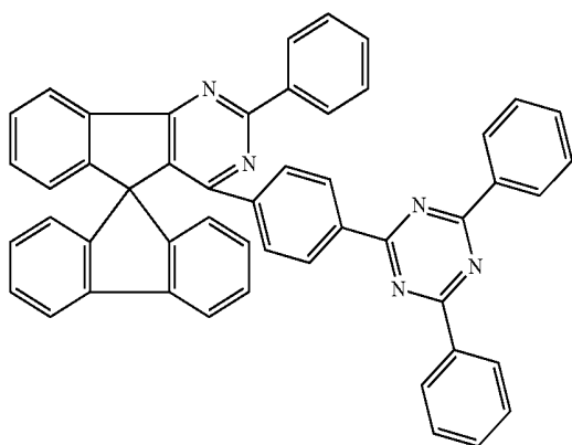
Chemical Formula 1-89
