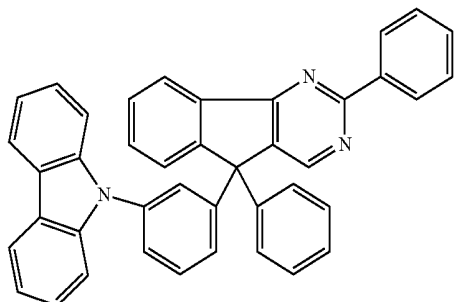
Chemical Formula 2-1
