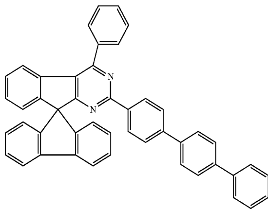
Chemical Formula 1-60
