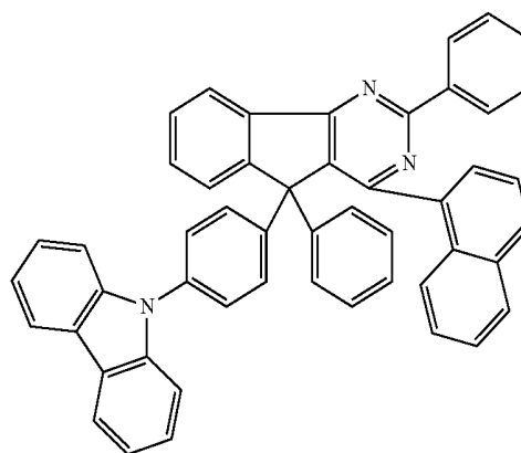
Chemical Formula 2-13
