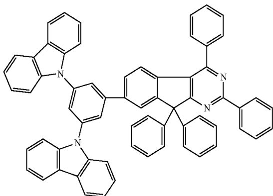
Chemical Formula 2-35
