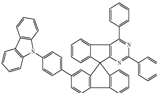
Chemical Formula 1-17
