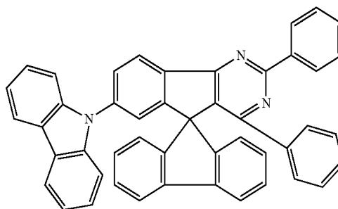
Chemical Formula 1-20
