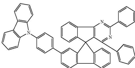
Chemical Formula 1-15
