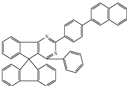
Chemical Formula 1-64
