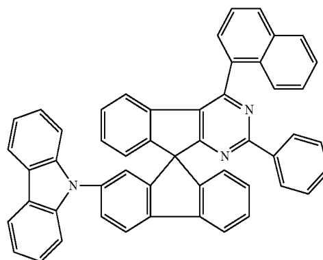
Chemical Formula 1-31
