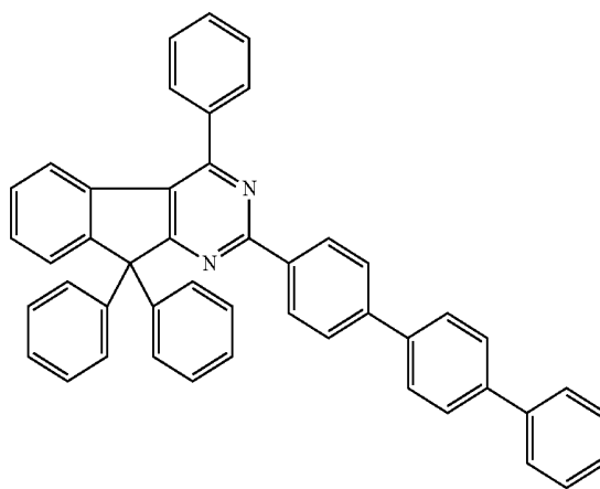
Chemical Formula 2-26
