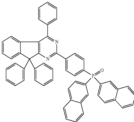
Chemical Formula 2-24
