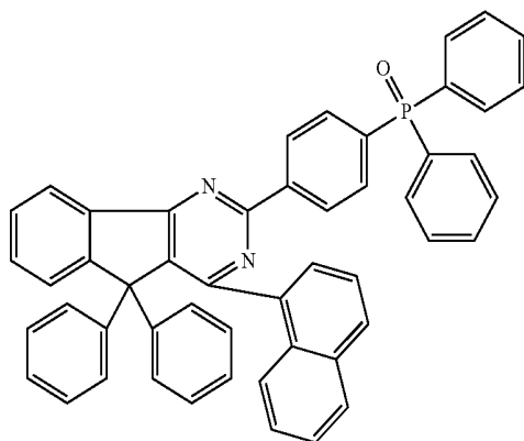
Chemical Formula 2-22
