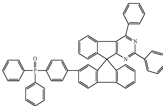
Chemical Formula 1-47
