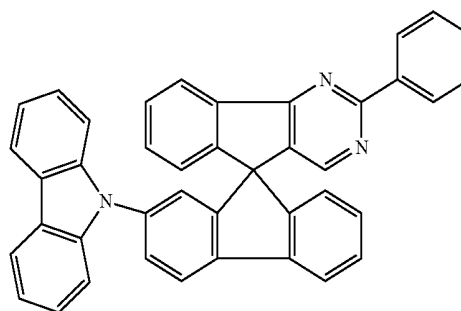
Chemical Formula 1-2
