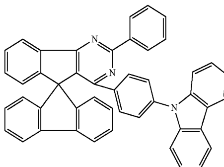
Chemical Formula 1-85
