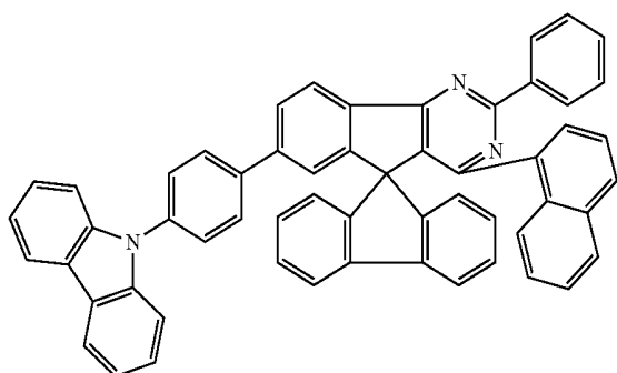
Chemical Formula 1-35
