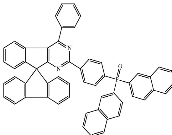
Chemical Formula 1-54
