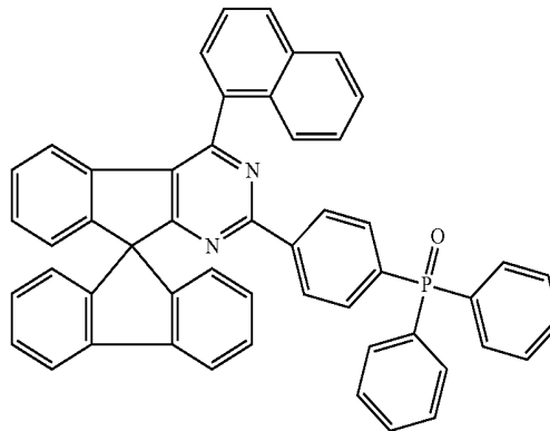
Chemical Formula 1-53
