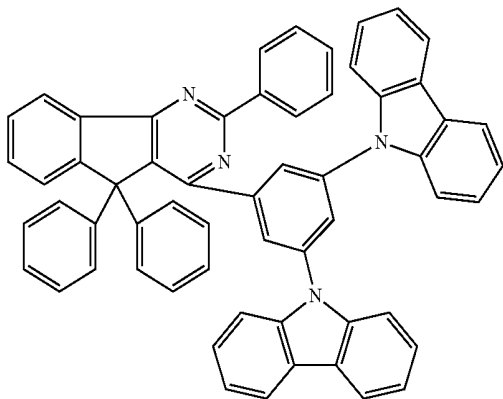
Chemical Formula 2-33
