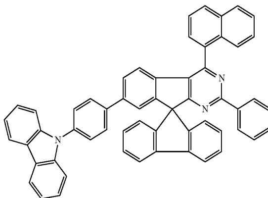
Chemical Formula 1-36
