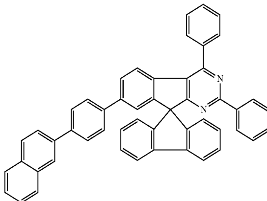
Chemical Formula 1-28
