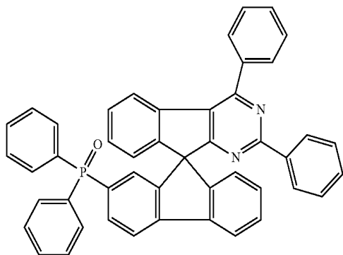
Chemical Formula 1-43
