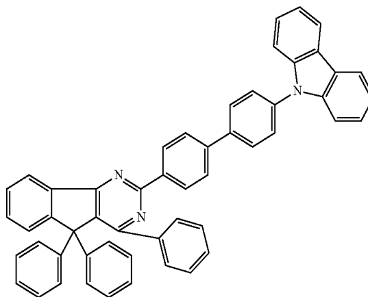
Chemical Formula 2-31
