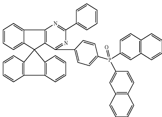
Chemical Formula 1-78
