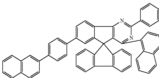
Chemical Formula 1-39
