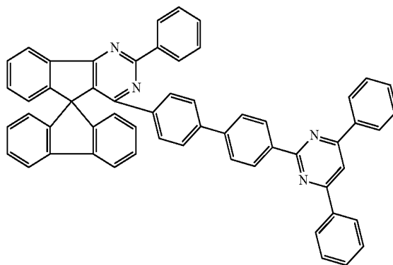
Chemical Formula 1-99
