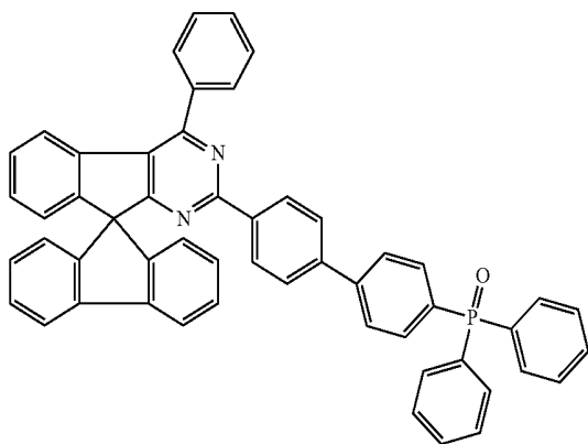
Chemical Formula 1-56
