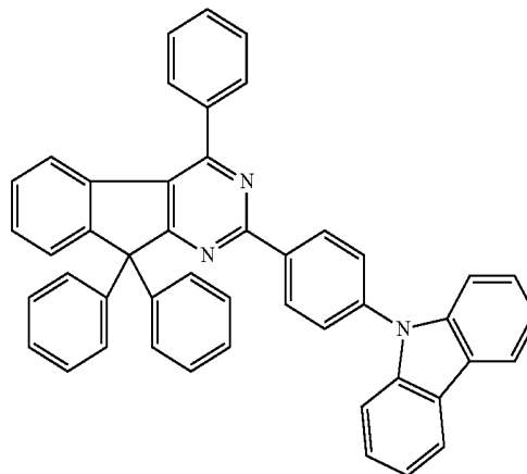
Chemical Formula 2-30
