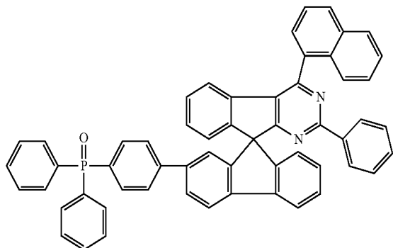
Chemical Formula 1-49
