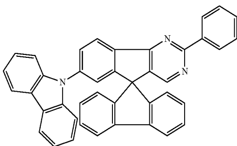
Chemical Formula 1-18
