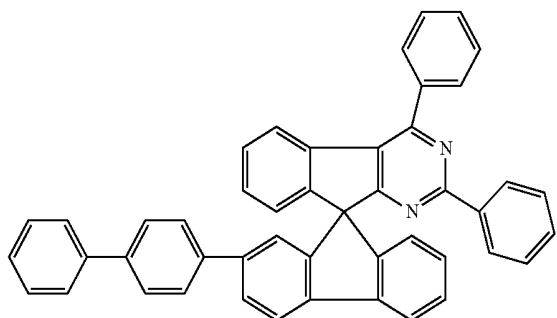
Chemical Formula 1-8
