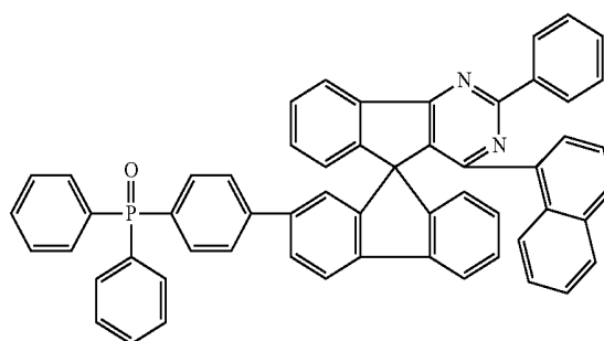
Chemical Formula 1-47
