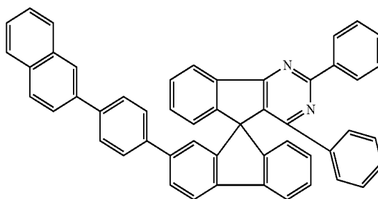
Chemical Formula 1-23
