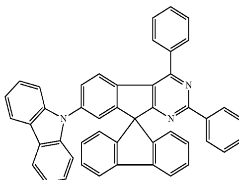
Chemical Formula 1-21
