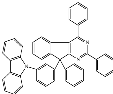
Chemical Formula 2-4
