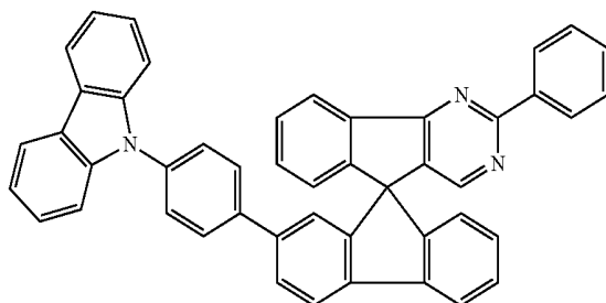
Chemical Formula 1-13
