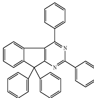
Chemical Formula 2-8
