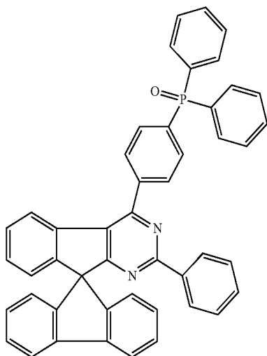
Chemical Formula 1-77
