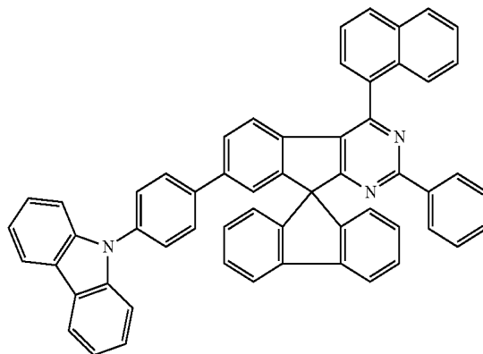
Chemical Formula 1-36
