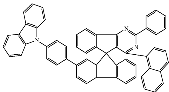
Chemical Formula 1-33
