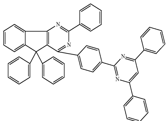
Chemical Formula 2-48
