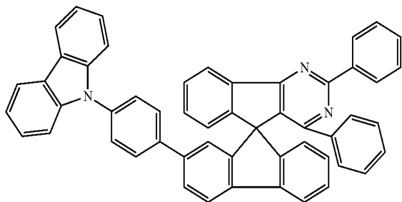
Chemical Formula 1-16
